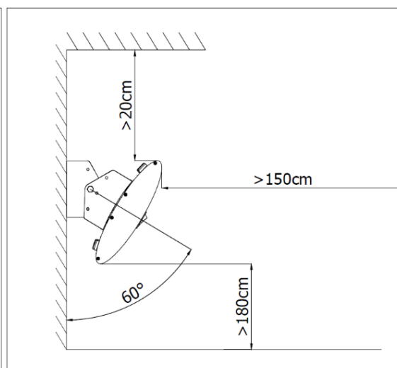
Wall installation:
